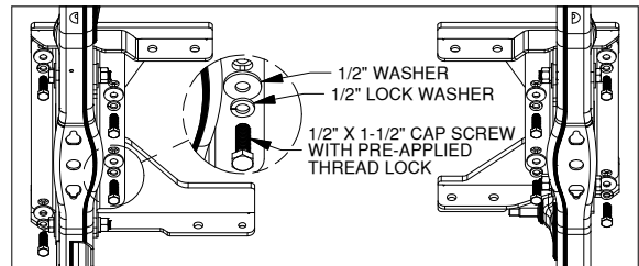
Figure B5: Bottom of truck frame looking up from the back of truck towards the cab
