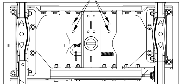
Figure F1: Bottom of truck bed looking up at hitch installation.
