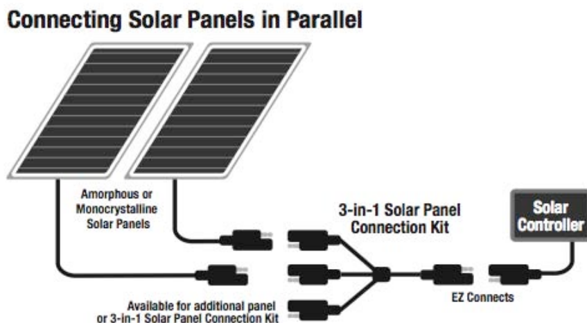
Figure 3. Wire Harness and Connections
