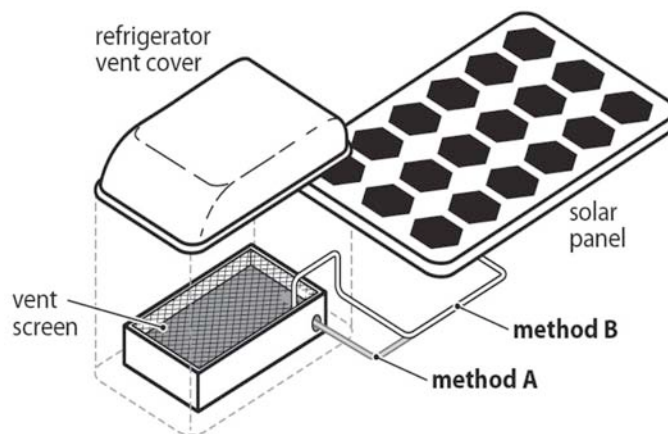
Figure 2. Wire Pair installed through Refrigerator Vent
