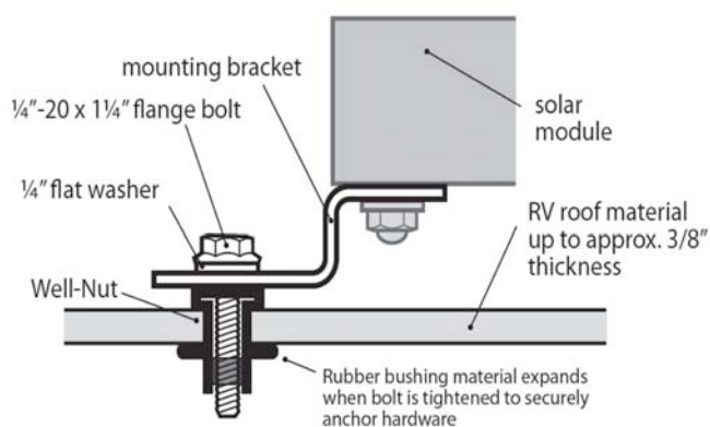
Figure 1. Mounting Bracket Assembly (Some bracket kits may vary)
