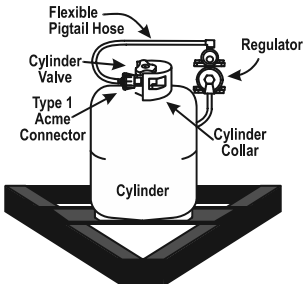
Fig. 7.5 Single cylinder
