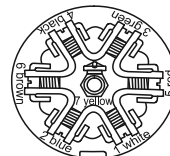
Fig. 4.2 7-way trailer plug - Car end, rear view
