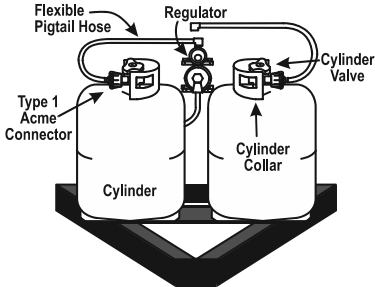
Fig. 7.6 Double cylinder
