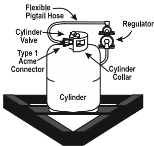
Fig. 7.5 Single cylinder
