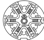
Fig. 4.2 7-way trailer plug - Car end, rear view
