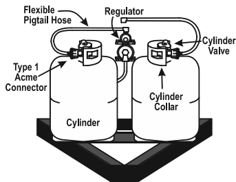
Fig. 7.6 Double cylinder
